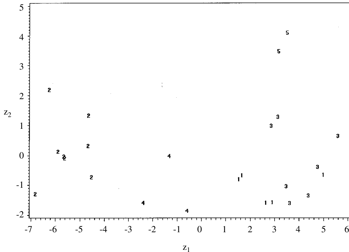
Figure 14.17. First two discriminant functions z_1 and z_2 for the clusters in Table 14.8.
