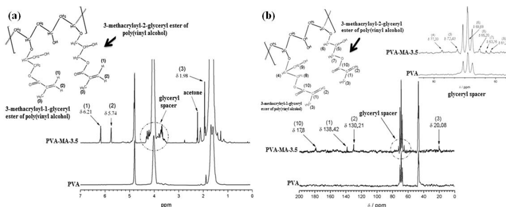
FIGURE 5. (a) ^1\text{H} NMR spectra of PVA and PVA-MA-3.5 for a coupling reaction at pH 3.5 (300 MHz, \text{D}_2\text{O} ). (b) ^{13}\text{C} NMR spectra of PVA and PVA-MA-3.5 for a coupling reaction at pH 3.5 (75.5 MHz, \text{D}_2\text{O} ).
