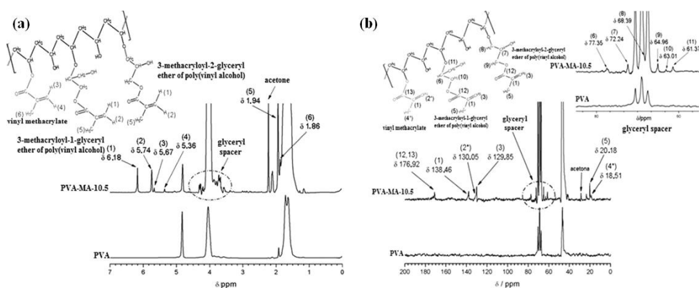
FIGURE 6. (a) ^1\text{H} NMR spectra of PVA and PVA-MA-10.5 for a coupling reaction at pH 10.5 (300 MHz, \text{D}_2\text{O} ), (b) ^{13}\text{C} NMR spectra of PVA and PVA-MA-10.5 for a coupling reaction at pH 10.5 (75.5 MHz, \text{D}_2\text{O} ).
