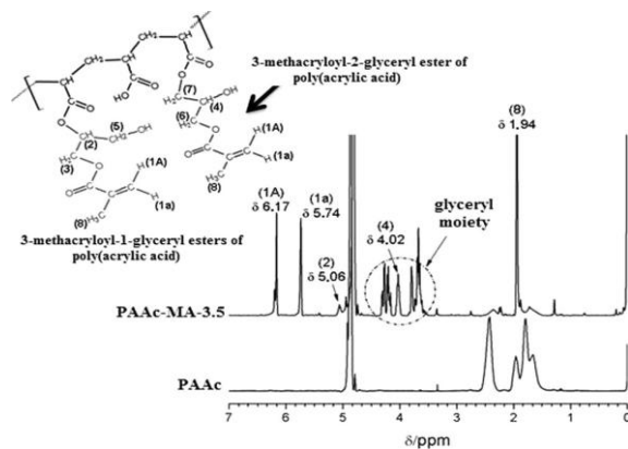
FIGURE 2. ^1\text{H} NMR spectra of PAAc and PAAc-MA-3.5 for a coupling reaction at pH 3.5 (300 MHz, \text{D}_2\text{O} ).
