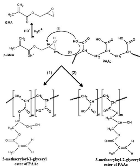
FIGURE 4. Schema of the coupling reaction of GMA with PAAc in an aqueous solution at pH 3.5 via an epoxide ring-opening mechanism.
