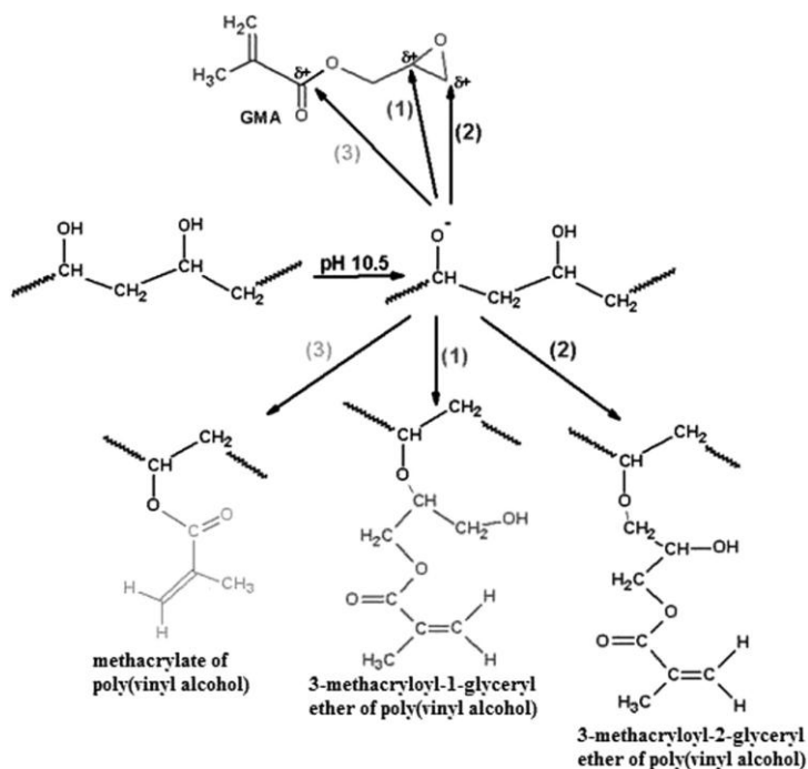
FIGURE 7. Schema of the reaction of GMA with PVA in an aqueous solution at pH 10.5 through three mechanism routes.
