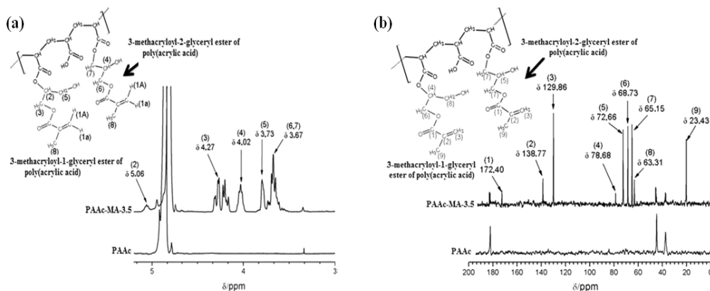
FIGURE 3. (a) Expanded ^1\text{H} NMR spectra of PAAc and PAAc-MA-3.5 in the spectral region of \delta 5-3, for a coupling reaction at pH 3.5 (300 MHz, \text{D}_2\text{O} ); (b) ^{13}\text{C} NMR spectra of PAAc and PAAc-MA-3.5 for a coupling reaction at pH 3.5 (75.5 MHz, \text{D}_2\text{O} ).
