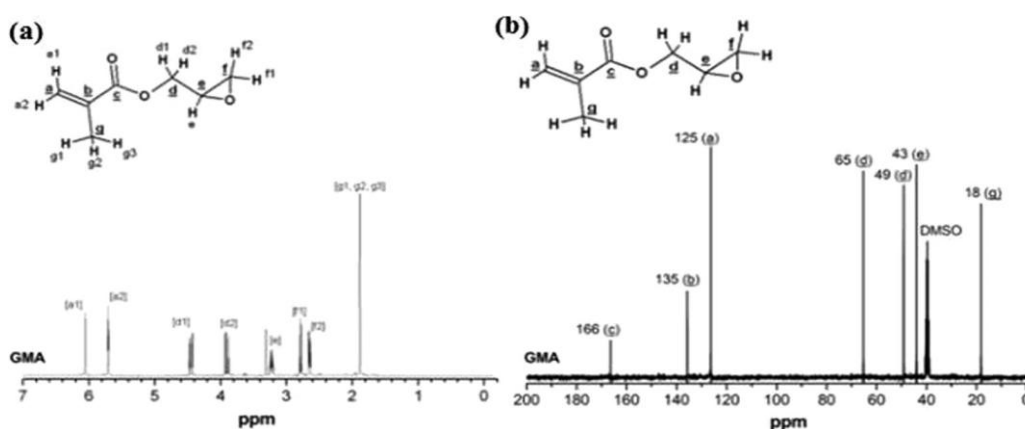
FIGURE 1. ^1\text{H} (a) and ^{13}\text{C} (b) NMR spectra of the pure GMA (DMSO- d_6 ).
